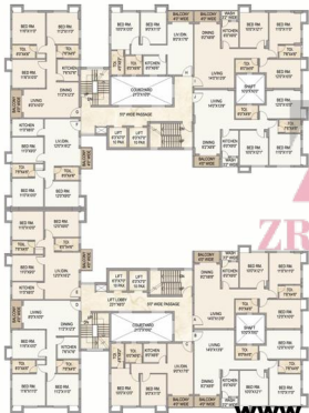
Typical Floor Plan - Plot - 1 (Block - 16)
